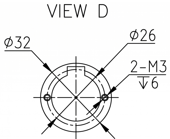
Mechanical View 4
