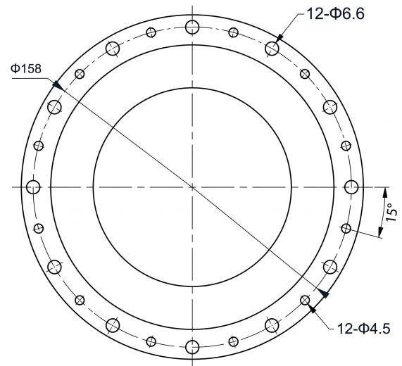
Mechanical View 2
