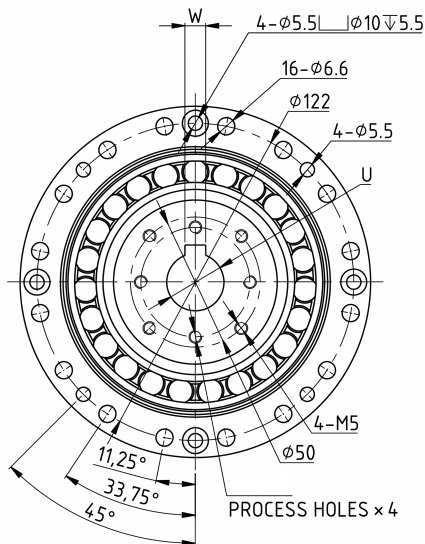
Mechanical View 3
