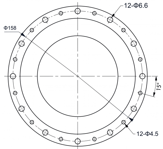
Mechanical View 2
