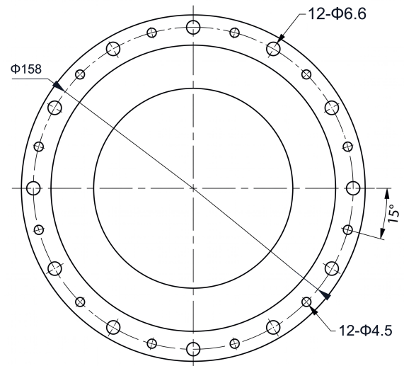
Mechanical View 2
