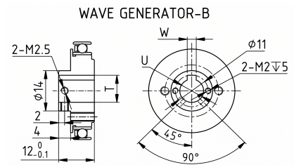
Mechanical View 4
