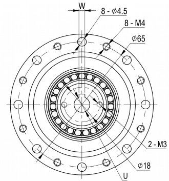
Mechanical View 2
