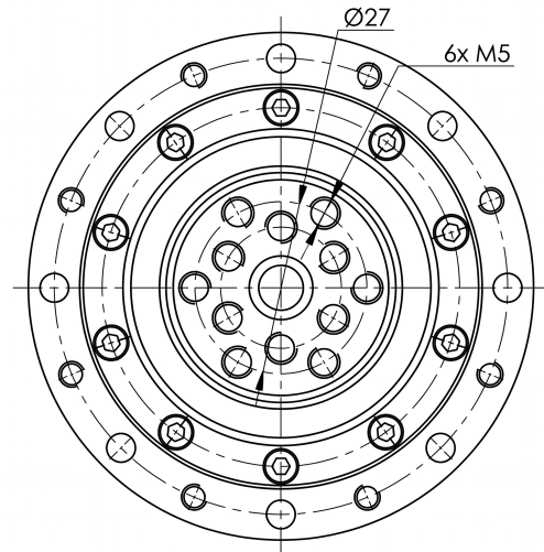
Mechanical View 2
