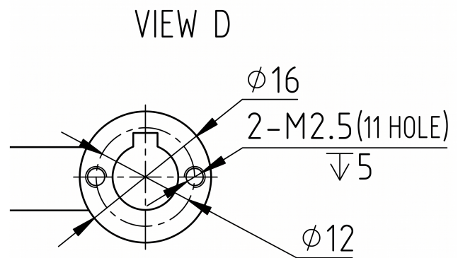
Mechanical View 4
