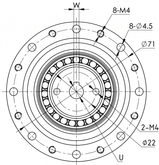
Mechanical View 3
