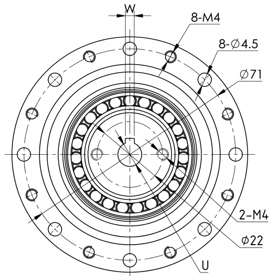
Mechanical View 3
