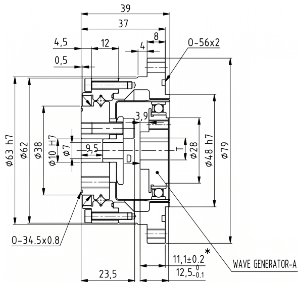
Mechanical View 1
