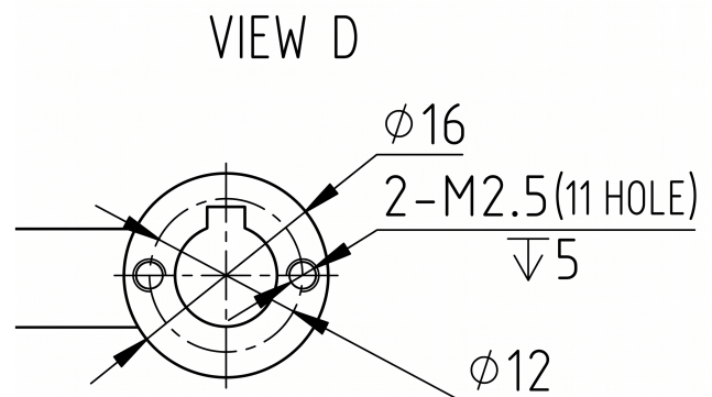
Mechanical View 4
