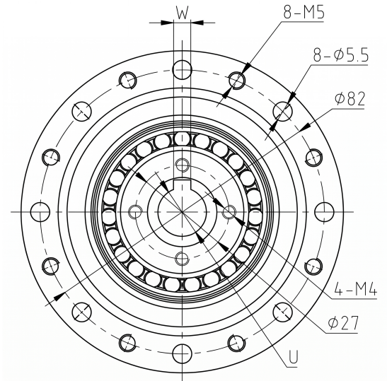
Mechanical View 2
