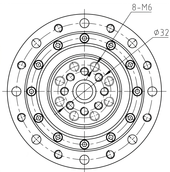
Mechanical View 3
