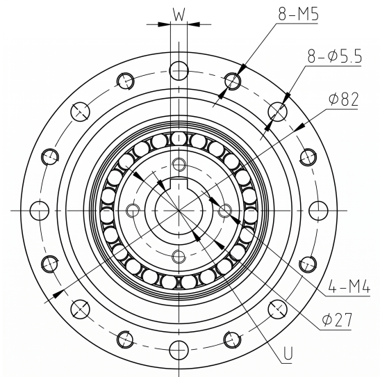
Mechanical View 2
