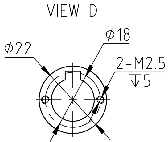
Mechanical View 4
