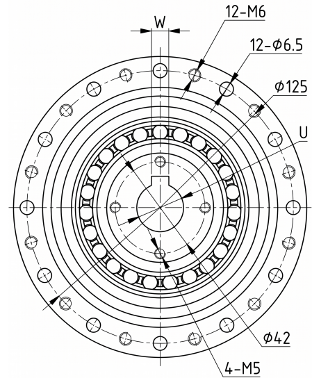
Mechanical View 2
