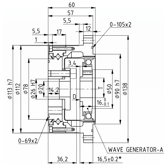
Mechanical View 1
