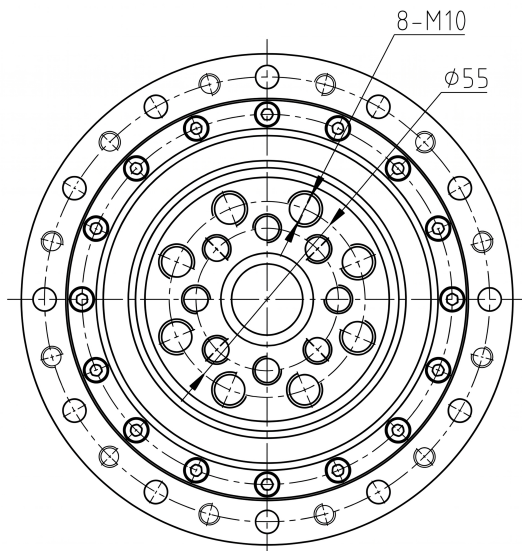
Mechanical View 3
