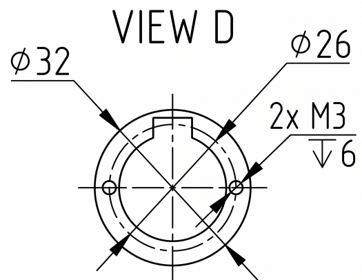
Mechanical View 4
