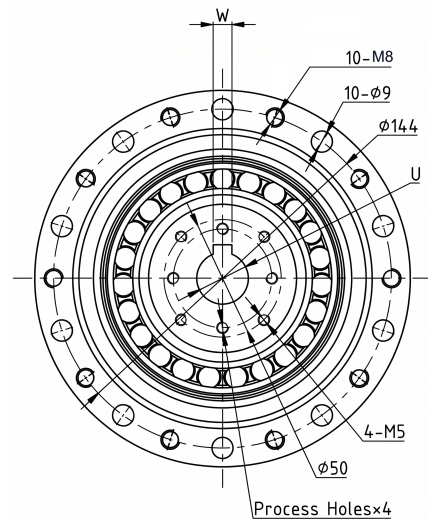
Mechanical View 2
