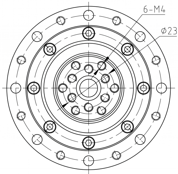
Mechanical View 3
