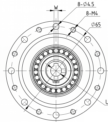
Mechanical View 2
