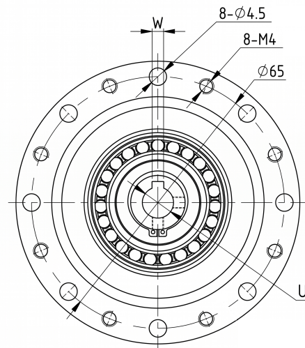
Mechanical View 2
