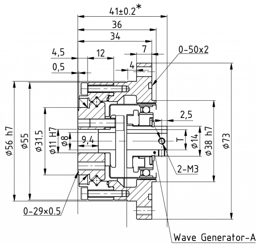
Mechanical View 1
