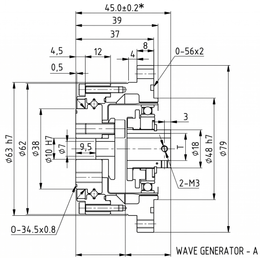
Mechanical View 1
