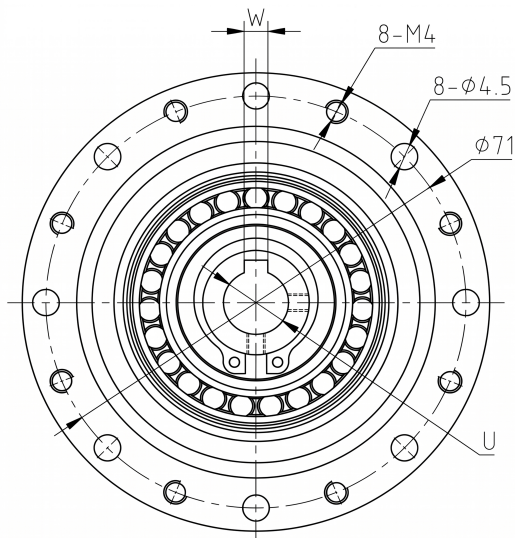
Mechanical View 3
