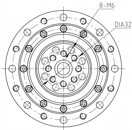
Mechanical View 3
