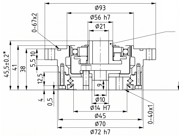
Mechanical View 1
