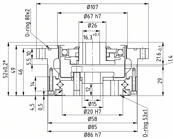
Mechanical View 1
