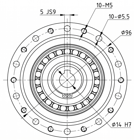
Mechanical View 2
