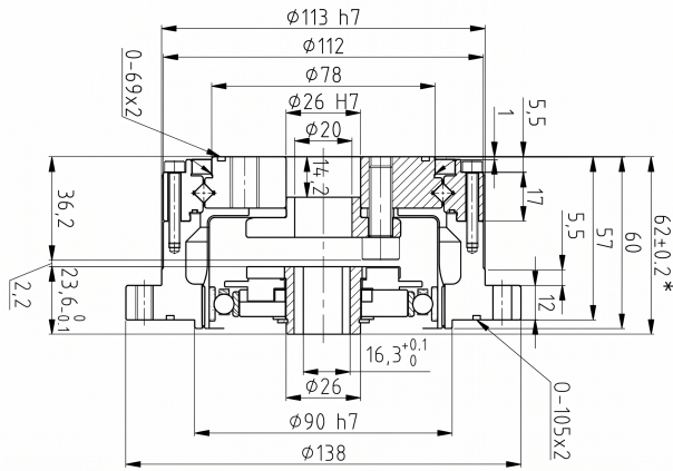
Mechanical View 1
