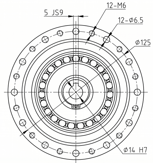
Mechanical View 2
