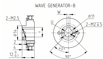
Mechanical View 4
