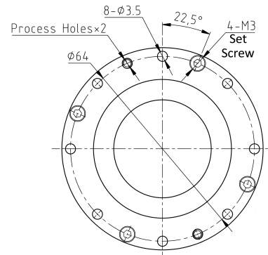
Mechanical View 2
