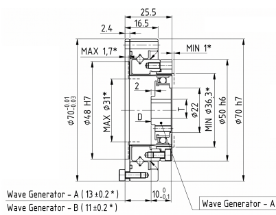
Mechanical View 3
