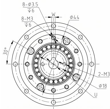
Mechanical View 1
