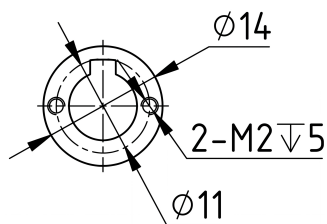
Mechanical View 5
