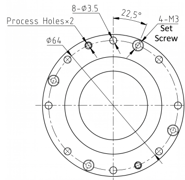
Mechanical View 2
