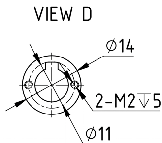
Mechanical View 5
