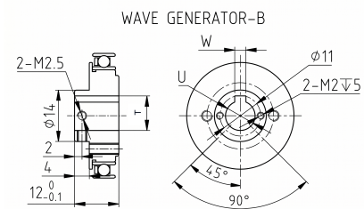
Mechanical View 4
