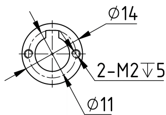
Mechanical View 5
