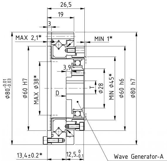
Mechanical View 1
