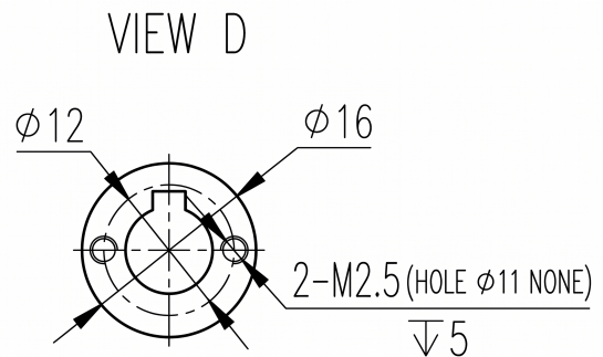
Mechanical View 4
