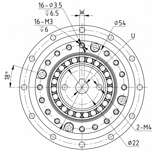
Mechanical View 2
