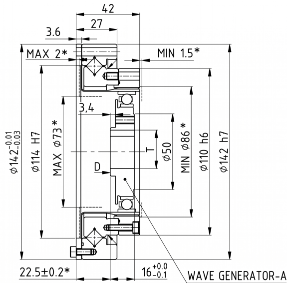
Mechanical View 3
