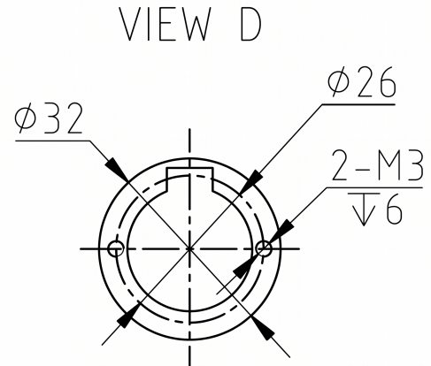
Mechanical View 4
