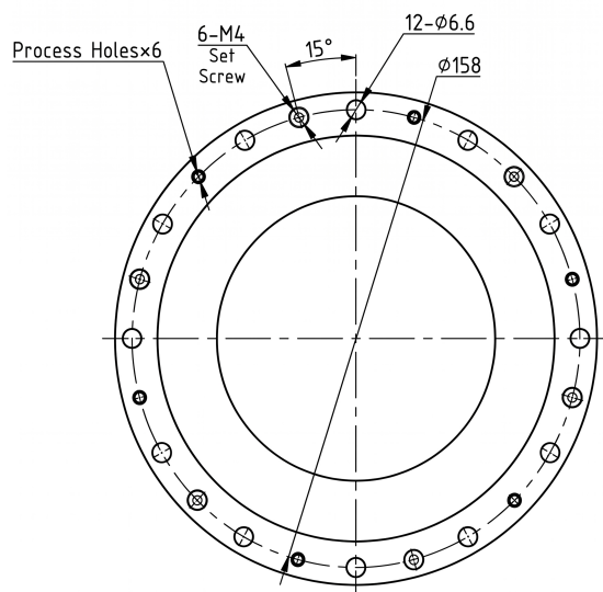
Mechanical View 3
