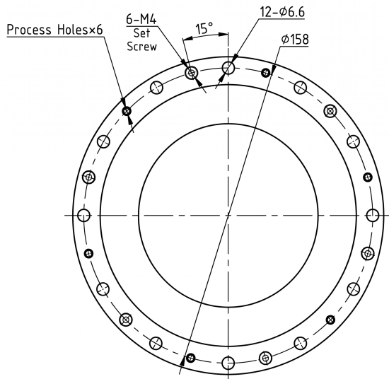
Mechanical View 3
