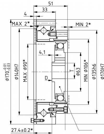
Mechanical View 2
