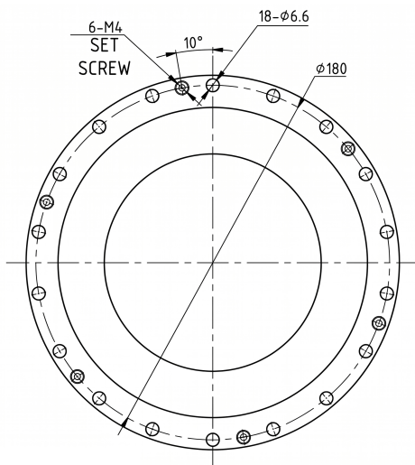
Mechanical View 3
