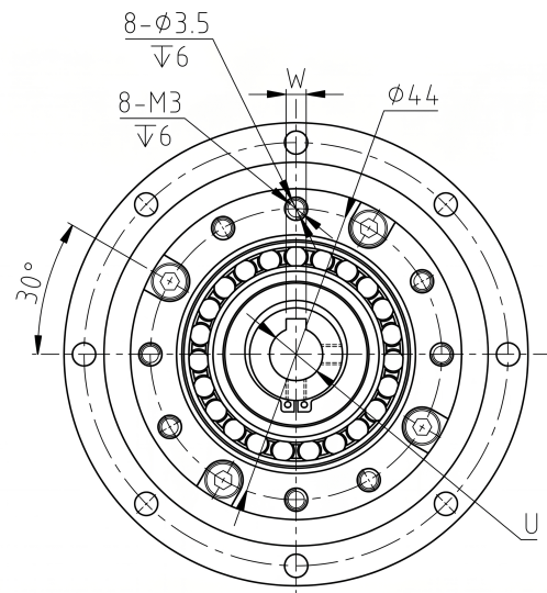
Mechanical View 2
