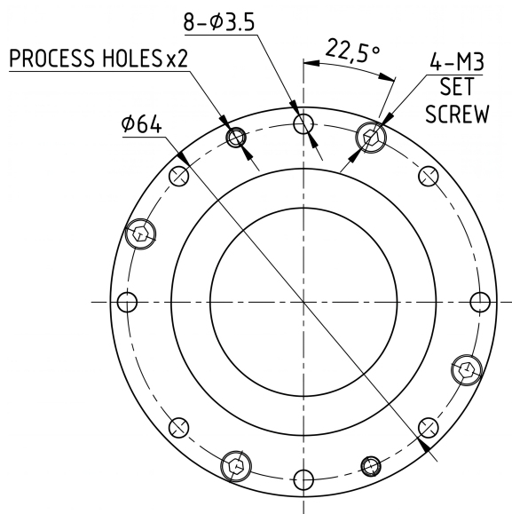
Mechanical View 3
