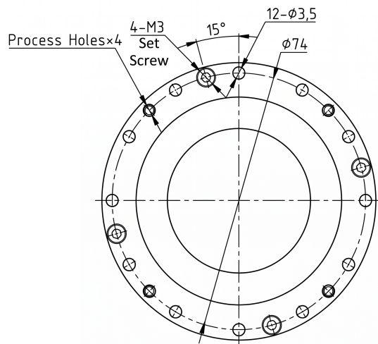
Mechanical View 3
