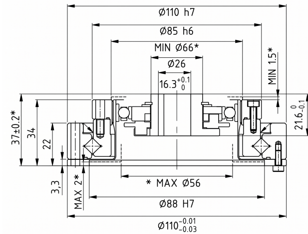
Mechanical View 1
