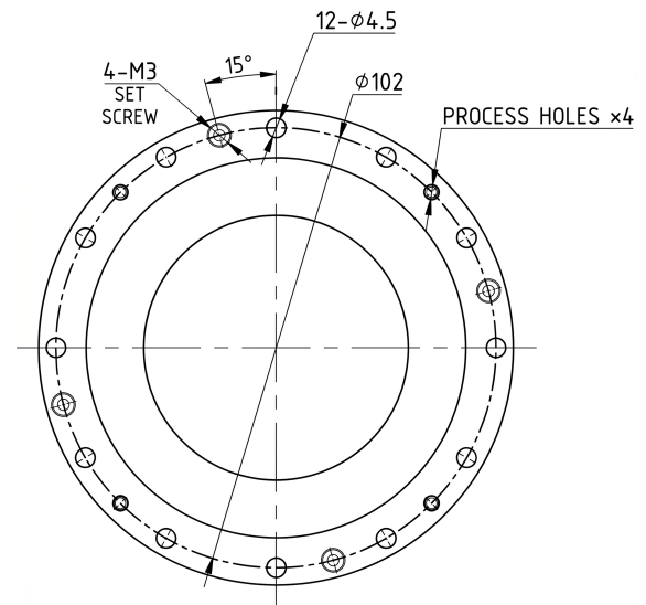
Mechanical View 2
