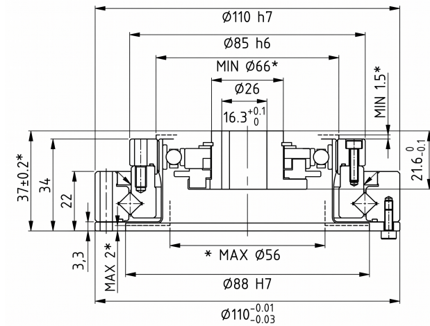
Mechanical View 1
