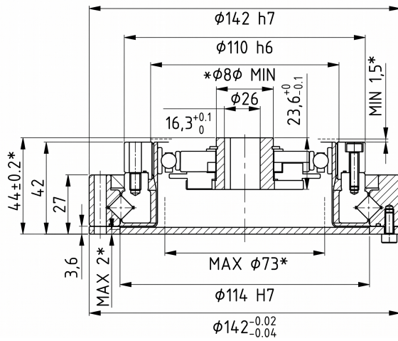
Mechanical View 1
