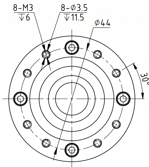
Mechanical View 3
