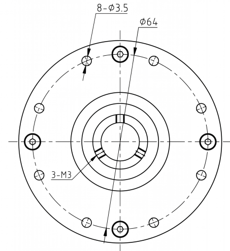
Mechanical View 2
