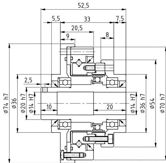
Mechanical View 1
