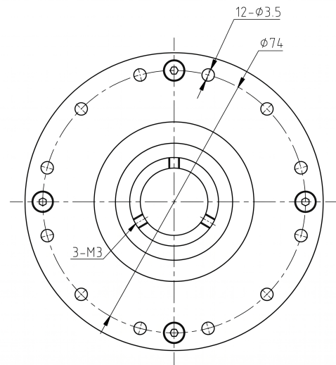
Mechanical View 2
