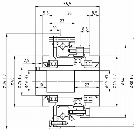
Mechanical View 1
