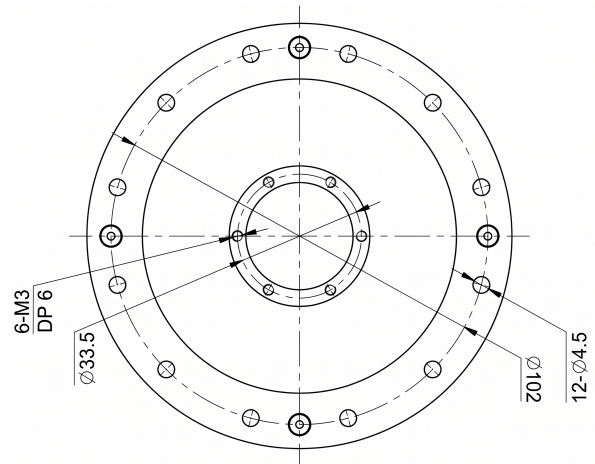
Mechanical View 2
