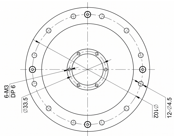
Mechanical View 2
