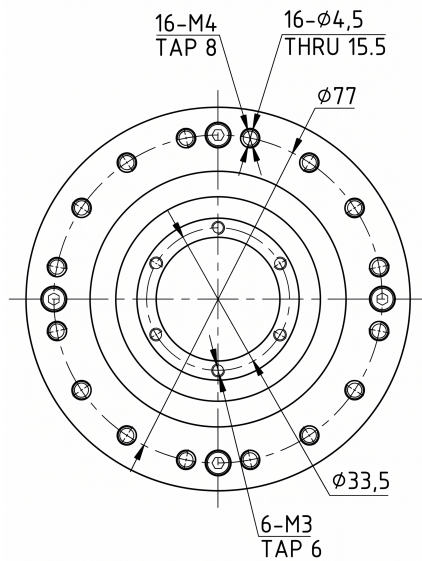
Mechanical View 3
