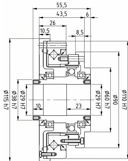
Mechanical View 1
