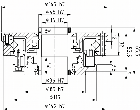
Mechanical View 1
