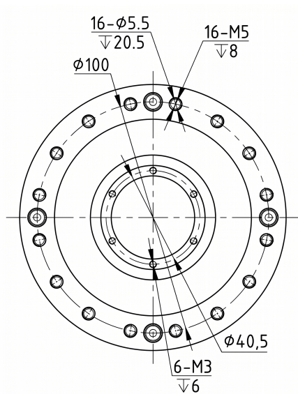
Mechanical View 3
