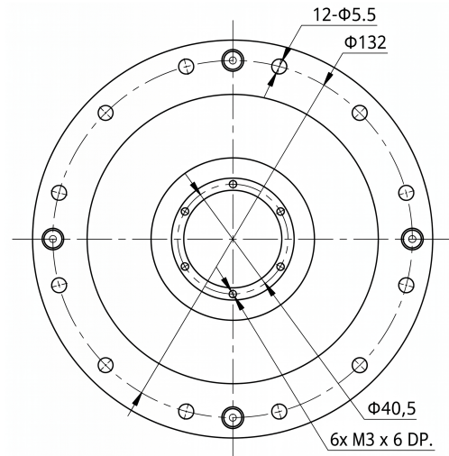
Mechanical View 2
