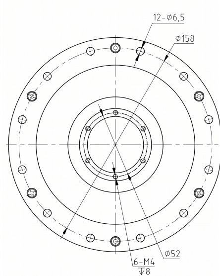
Mechanical View 2
