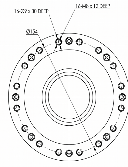
Mechanical View 3
