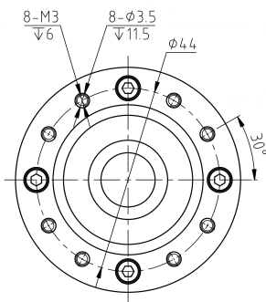
Mechanical View 4
