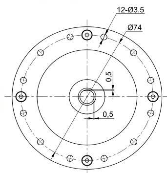
Mechanical View 7
