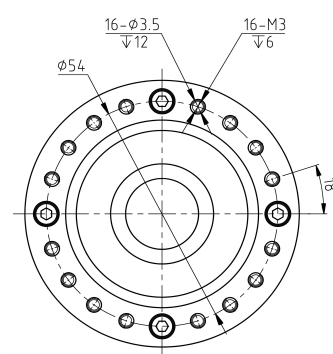
Mechanical View 8
