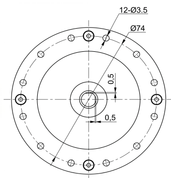
Mechanical View 7
