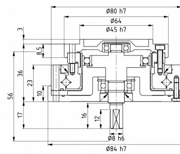
Mechanical View 6
