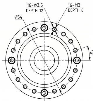
Mechanical View 4
