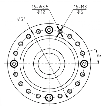
Mechanical View 8
