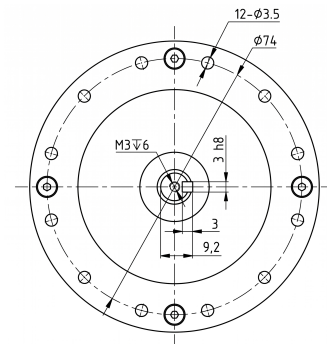
Mechanical View 3
