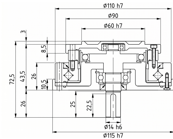
Mechanical View 1
