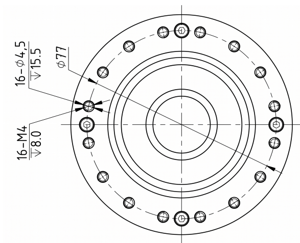
Mechanical View 3
