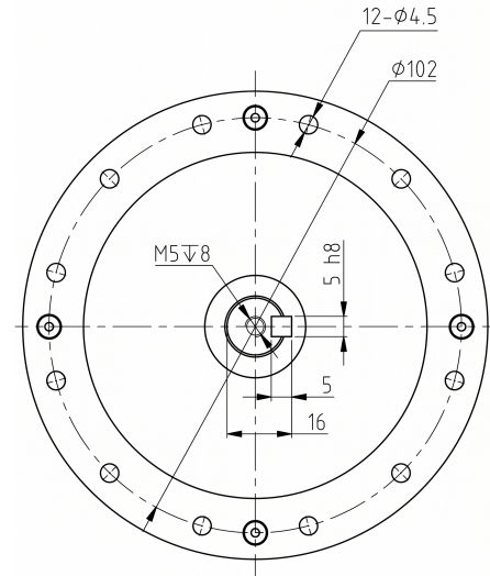
Mechanical View 2
