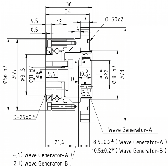
Mechanical View 1
