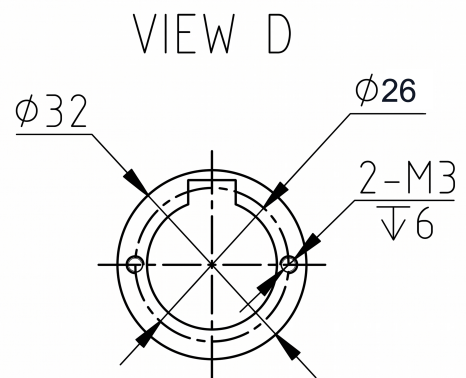
Mechanical View 4
