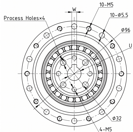
Mechanical View 2
