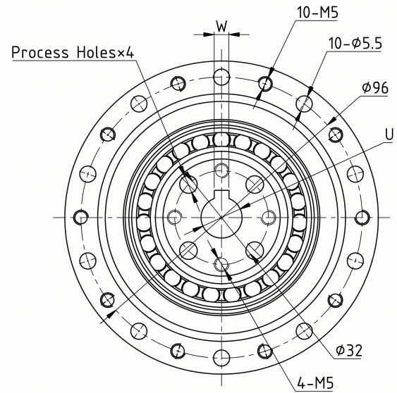
Mechanical View 2
