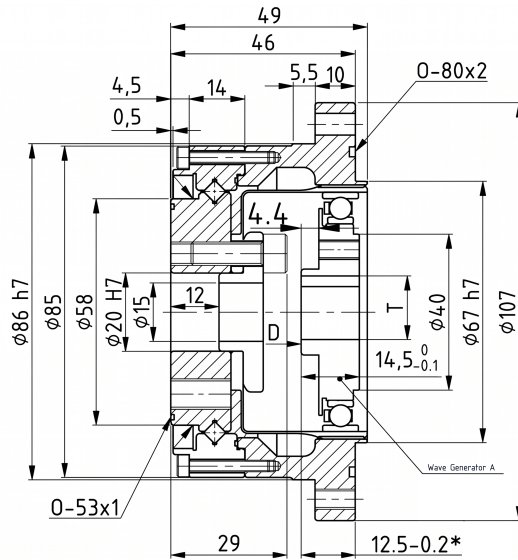
Mechanical View 1
