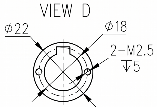
Mechanical View 4
