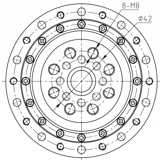
Mechanical View 3
