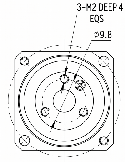
Mechanical View 1
