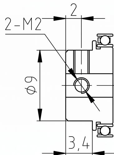
Mechanical View 4
