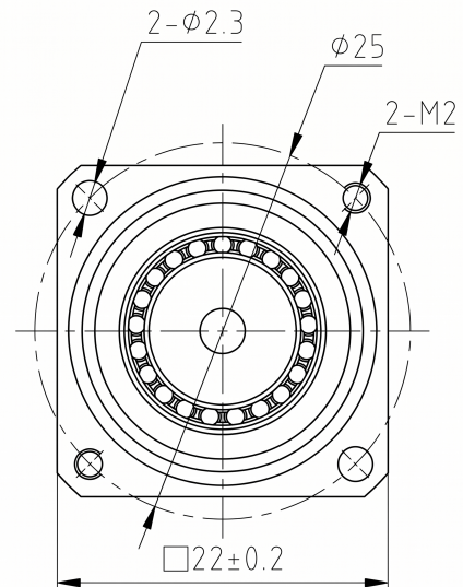
Mechanical View 2
