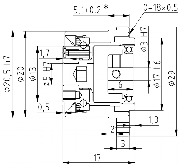
Mechanical View 3
