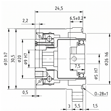
Mechanical View 1
