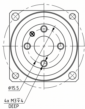
Mechanical View 3
