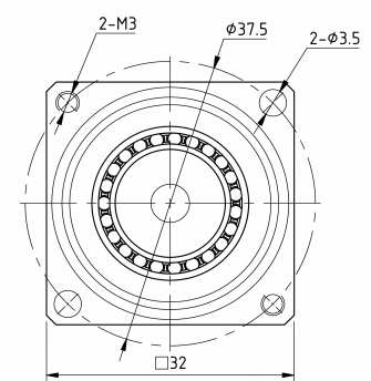
Mechanical View 2
